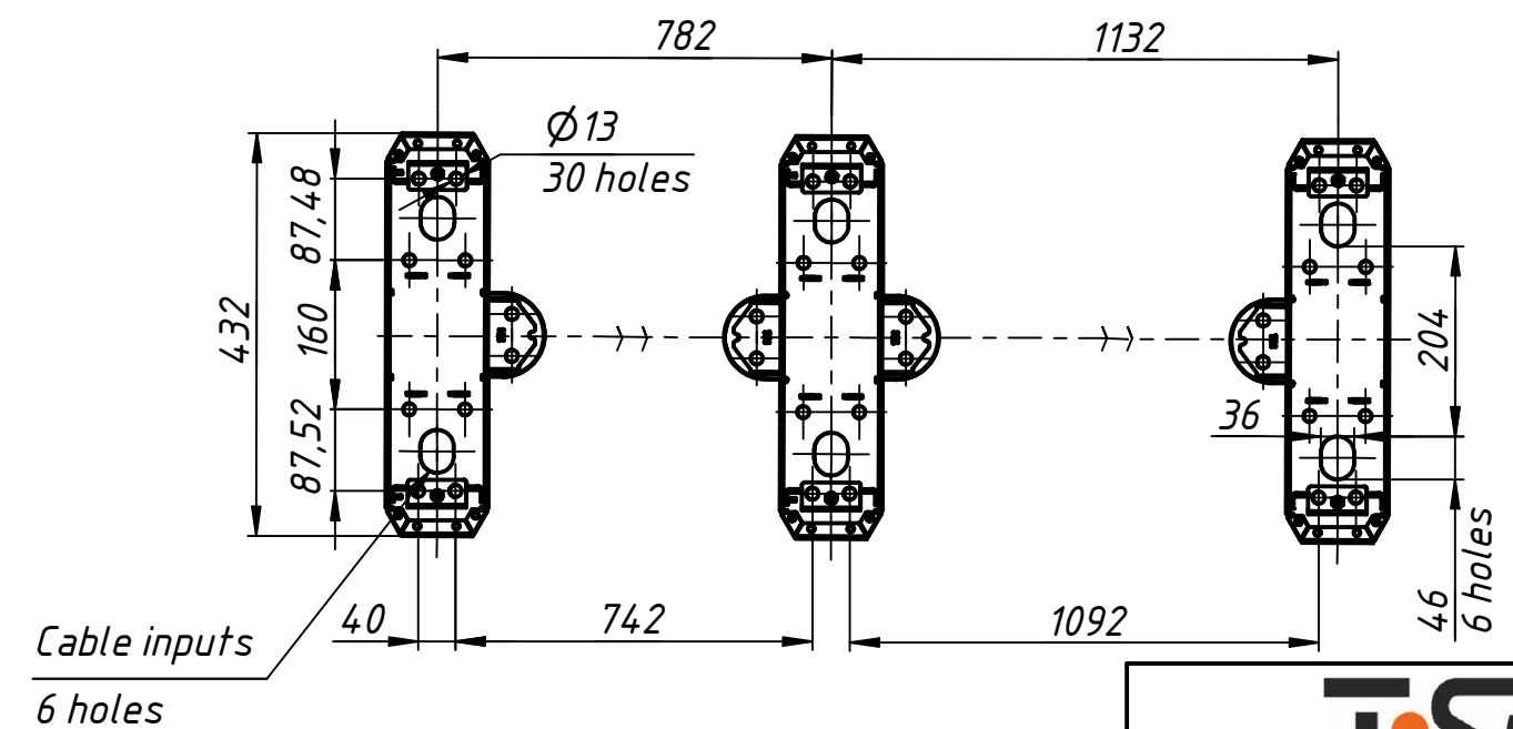
Installation tamplate
